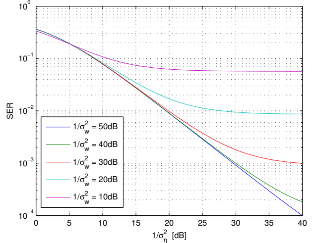
Fig. 4. SER with ICSI for \alpha = 1 and \sigma_h = 1 .
